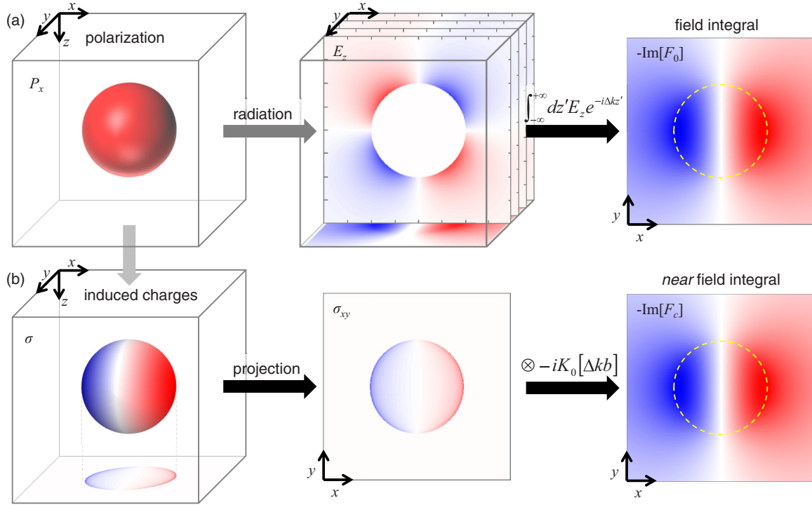
FIG. 1. (Color online) Schemes of evaluating (a) the field integral \tilde{F}_0 by numerical integration of the electric field and (b) the near-field integral \tilde{F}_c by the convolution method. See text for notations.
