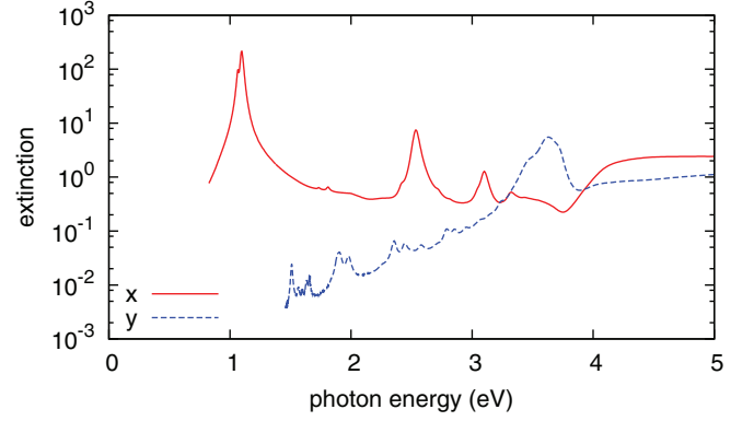
FIG. 3. (Color online) Optical extinction efficiencies of a silver nanorod at parallel ( \hat{x} , solid red line) and perpendicular ( \hat{y} , dashed blue line) polarizations.
